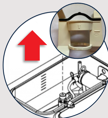
2. Remove current agitator paddle from both sides of the machine
