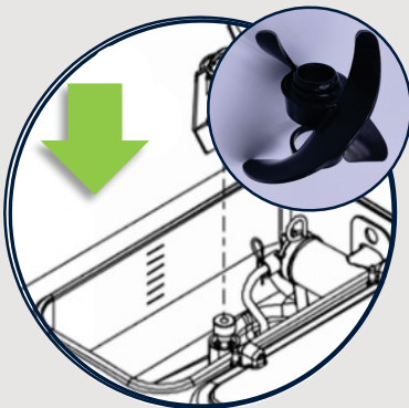
3. Replace with new agitator paddles
